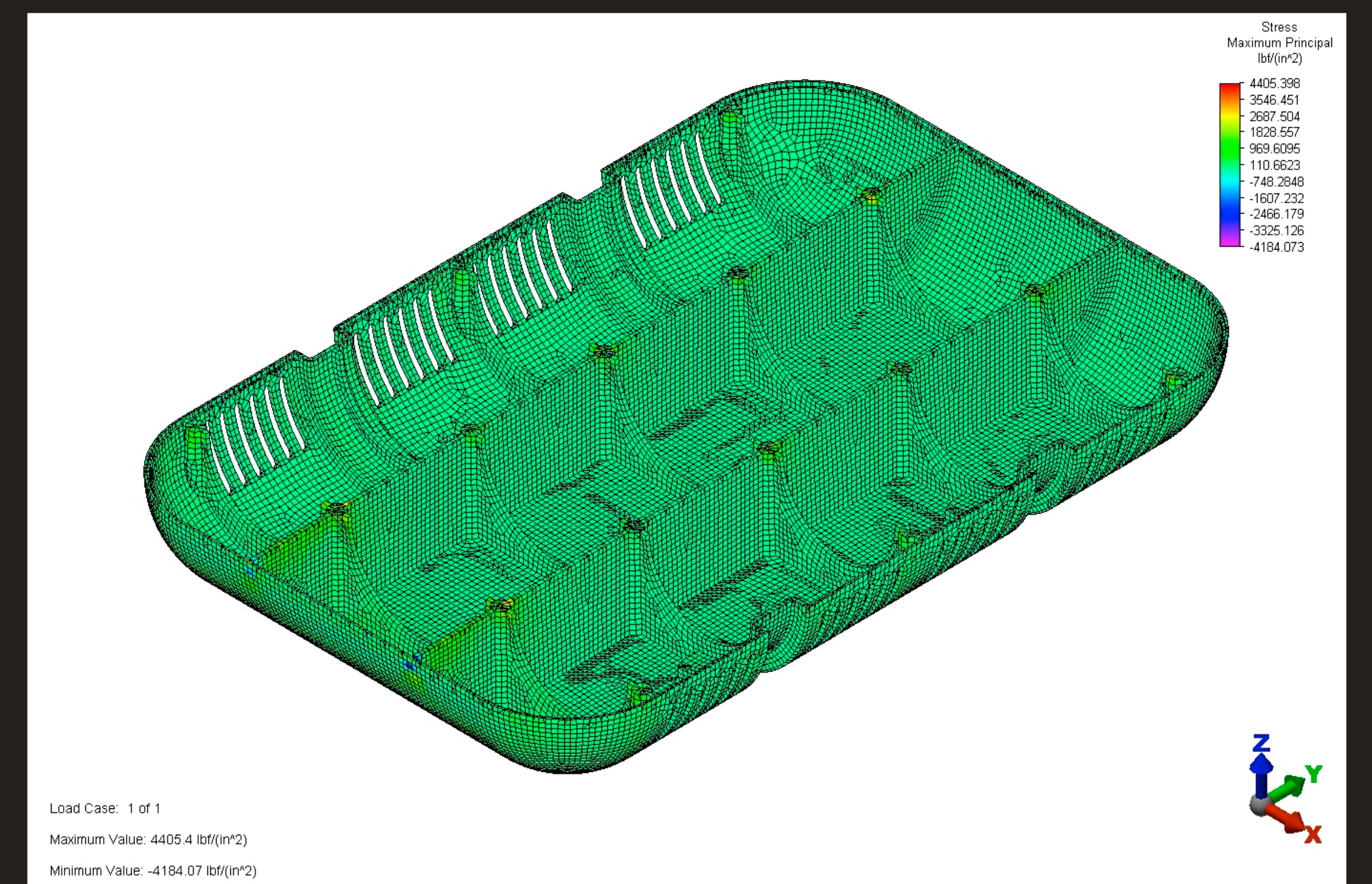
Bottom Impact Max Principal Stress
