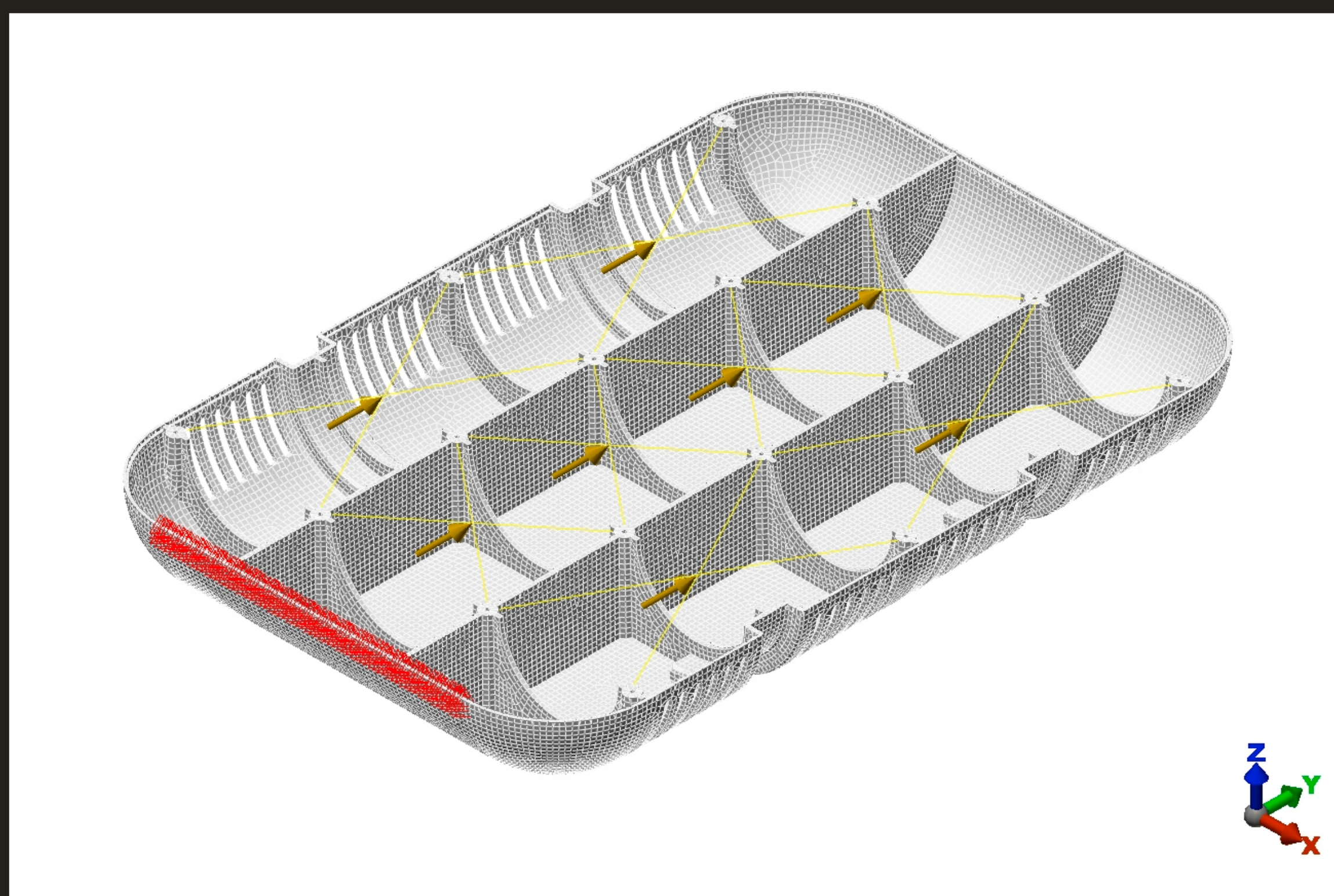
Algor Bottom Impact FEA Model + Concentrated Mass
