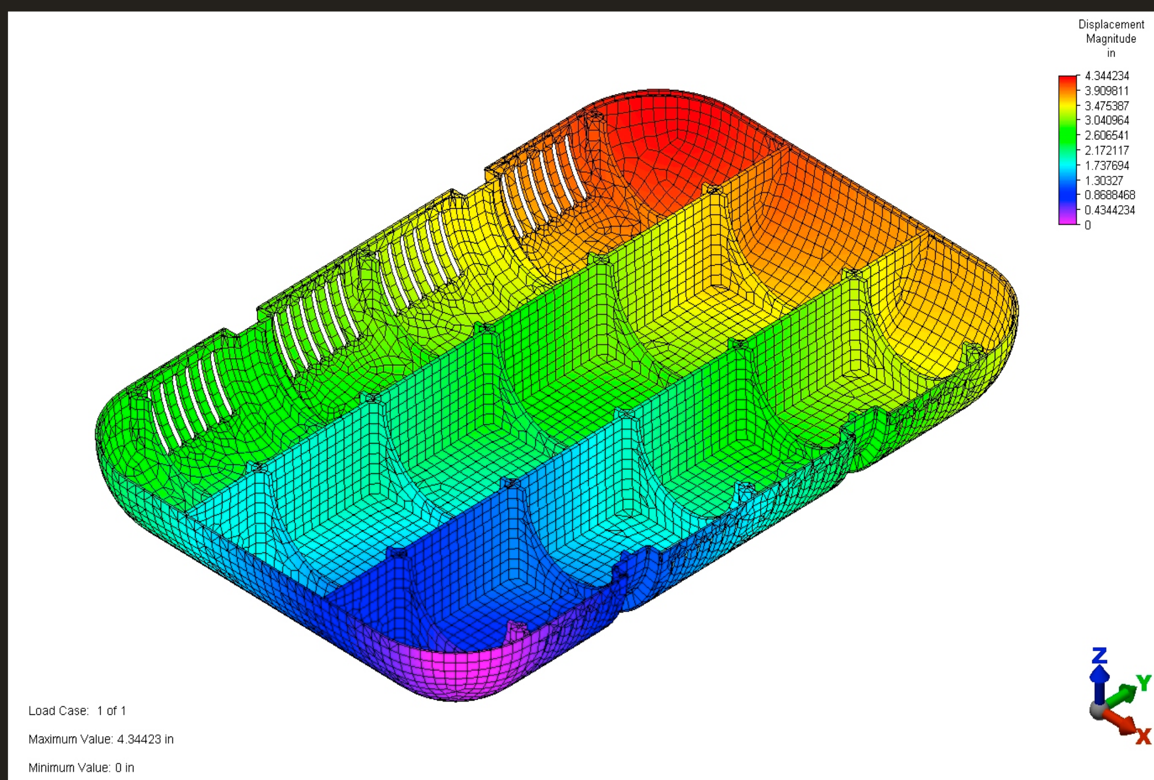
Corner Impact Displacement
