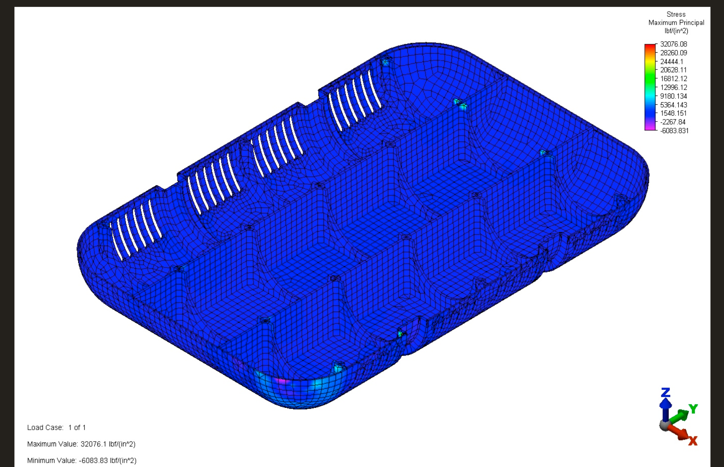
Corner Impact Max Principal Stress
